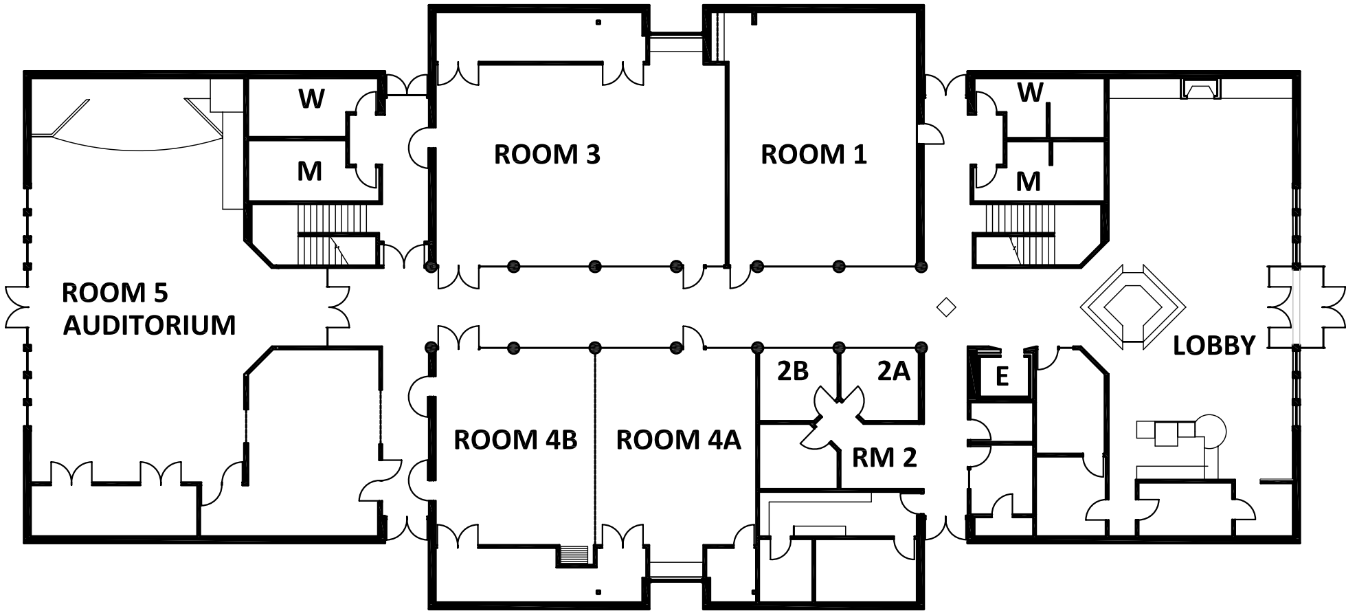
PERSON SENIOR WING FIRST FLOOR
