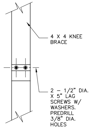
DETAIL "D"
